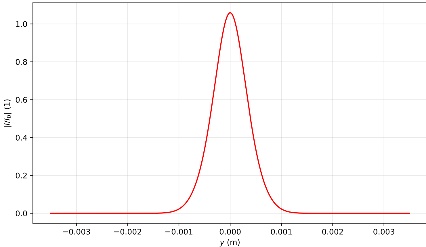
Intensity profile I(x=0, y, z=0.716)/I_0 , P_{in}=0.5P_{cr} , artificial time
